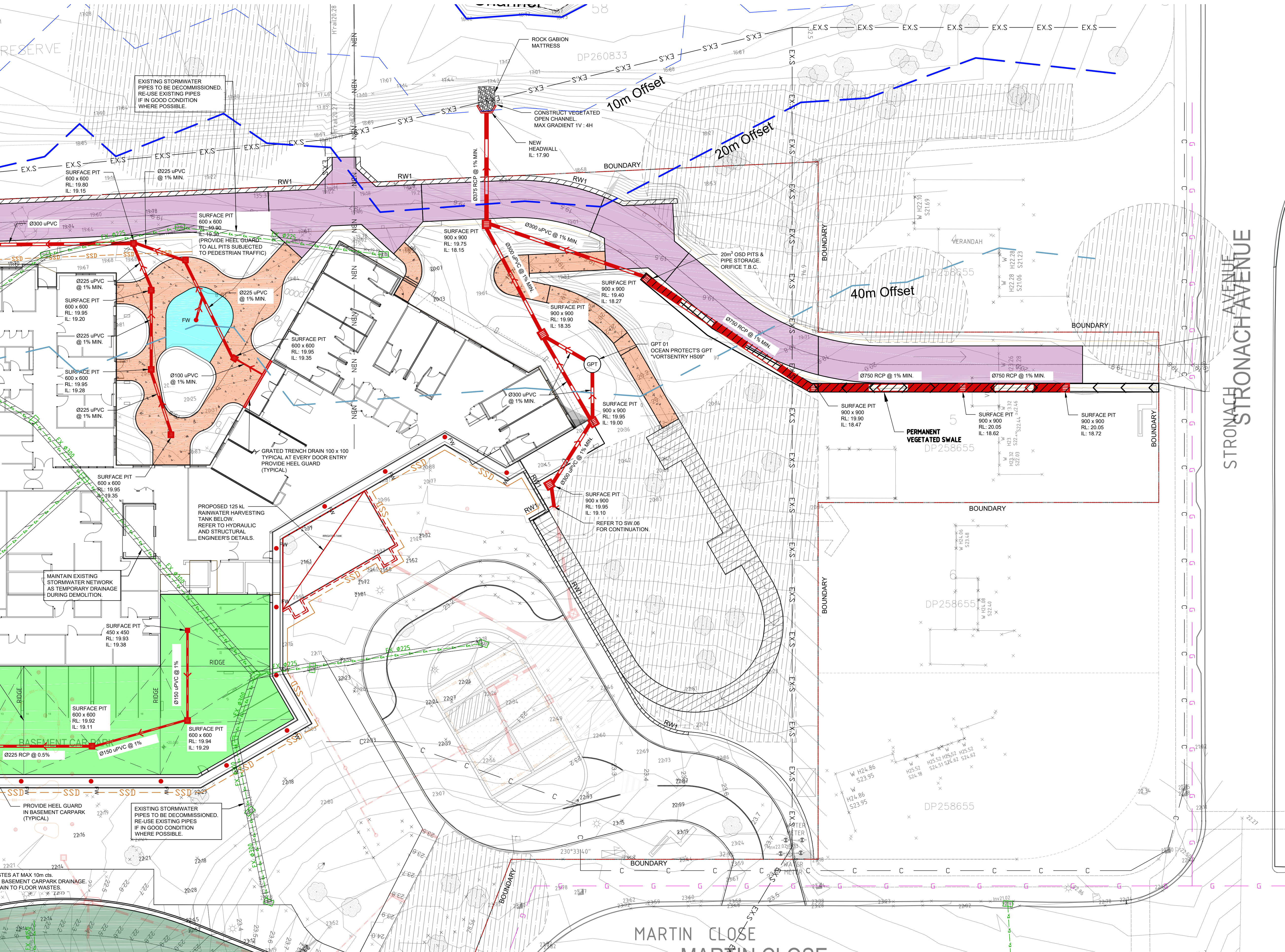
STORMWATER DRAINAGE CONCEPT PLAN - LOWER GROUND SHEET 02 SCALE 1:200
