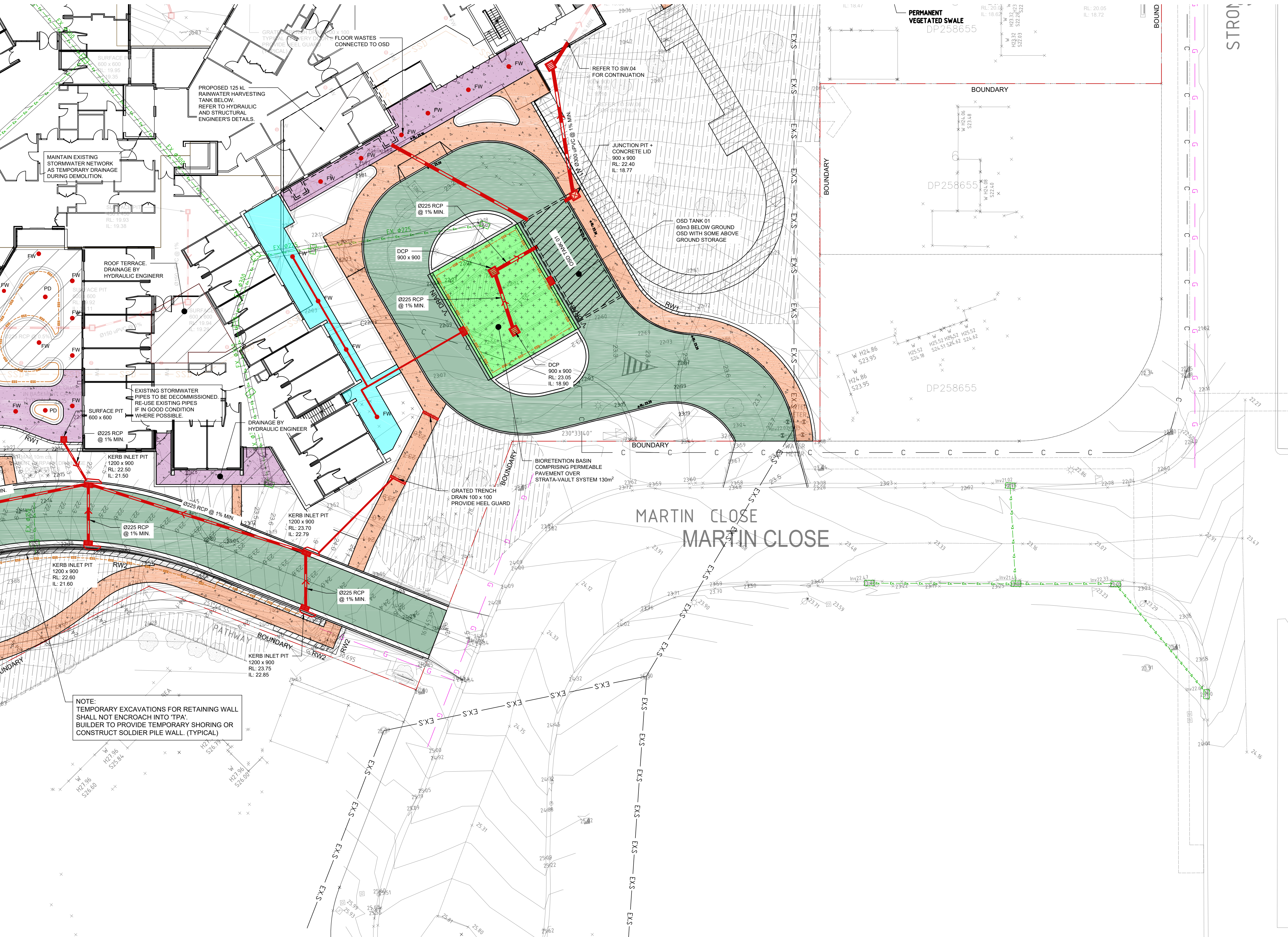
STORMWATER DRAINAGE CONCEPT PLAN - GROUND SHEET 02 SCALE 1:200
